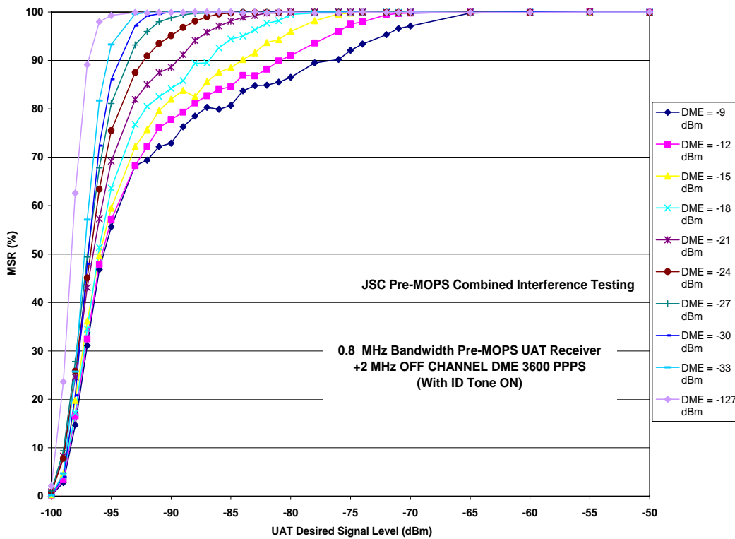
Figure D-9: UAT High Performance Receiver DME 3600 Pulse Pairs at +2 MHz
