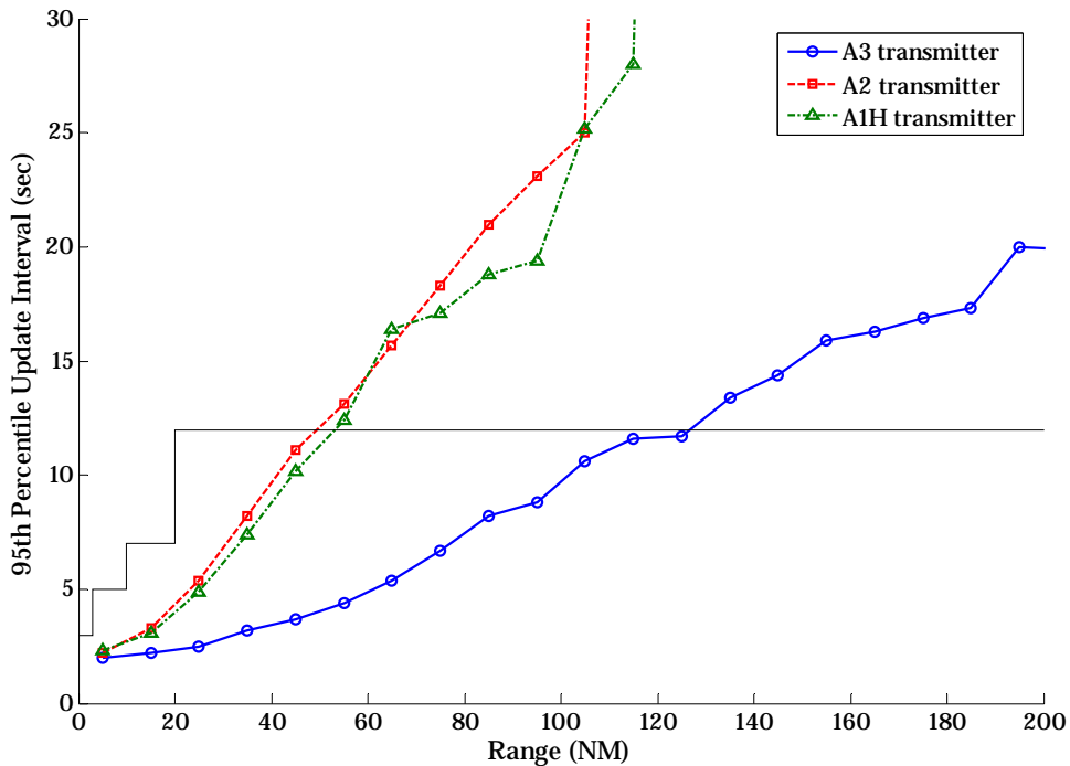
Figure B-23: Air-to-Air Reception by A3 Receiver at High Altitude over BRU in CE 2015
