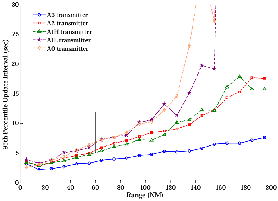
Figure B-30: Air-to-Ground Reception at BRU in CE 2015
