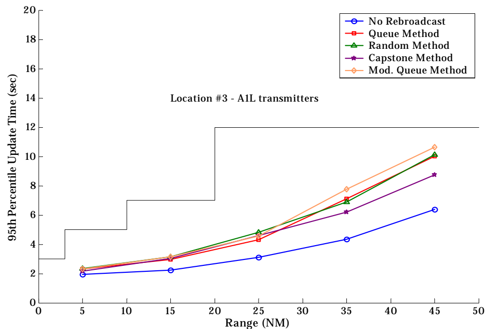
Figure B-41: ADS-B Air-to-Air Performance in the Presence of ADS-R Ground Transmissions in LA 2020
