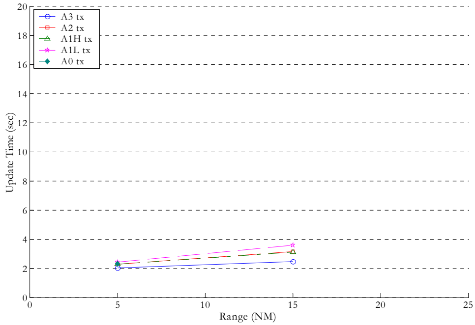
Figure B-36: A0 Receivers on the Ground in LA2020 Receiving All Aircraft on Approach at an Altitude of 2000 feet
