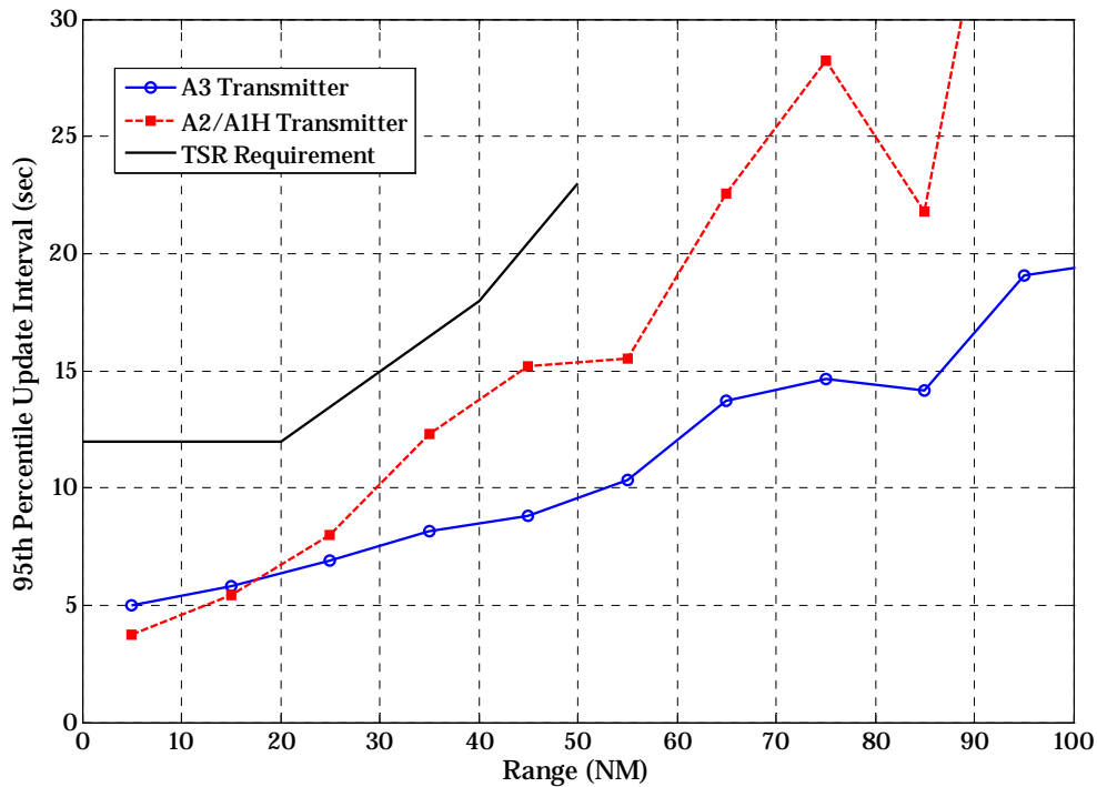
Figure B-22: 95 th Percentile Update Interval for Target State Reports as a Function of Range for A3 and A2/A1H Transmitters
