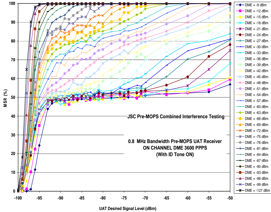
Figure D-13: UAT High Performance Receiver DME 3600 Pulse Pairs on Frequency
