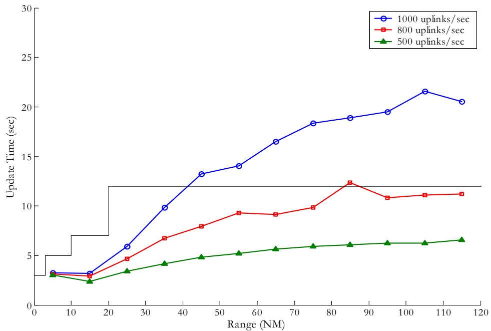
Figure B-44: 95 th Percentile State Vector Updates Times for an A3 Receiver at 40,000 feet Receiving A3 Transmissions in the Presence of a Ground Station 40 NM Away at Various Uplink Rates
