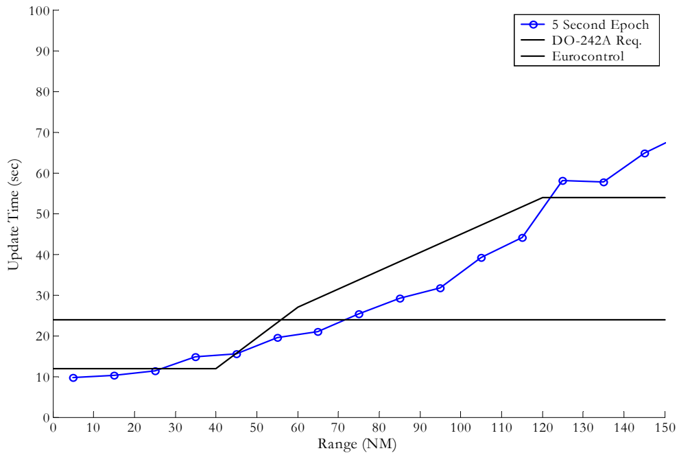
Figure I-2: 95th Percentile Trajectory Change Report Update Times for an A3 Receiver at High Altitude in CE 2015 over Brussels Using a 5 Second Epoch to Deliver 4 TC Messages
