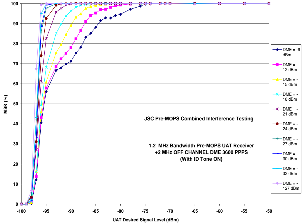
Figure D-8: UAT Standard Receiver Performance DME 3600 Pulse Pairs at +2 MHz
