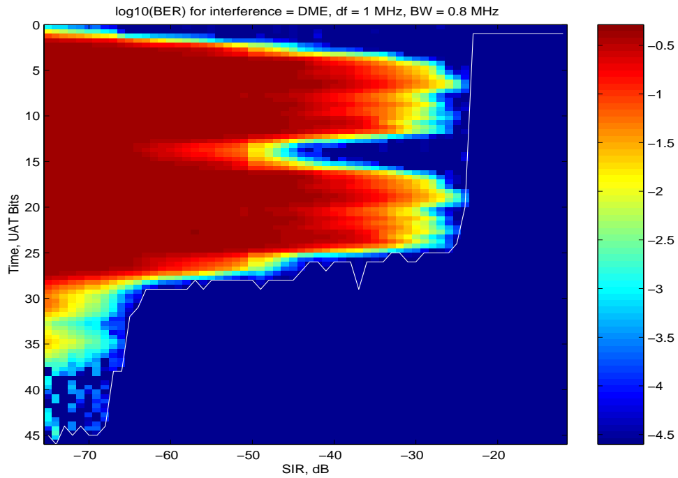
Figure B-4: BER Due to DME interference
