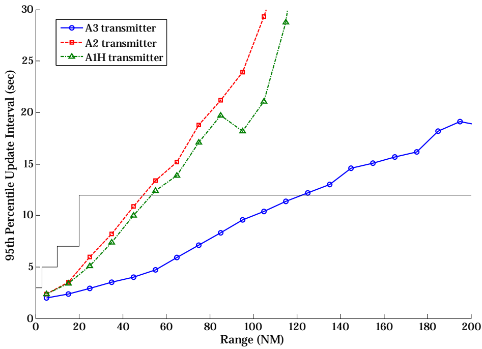
Figure B-13: Air-to-Air Reception by A3 Receiver at High Altitude over LA 2020
