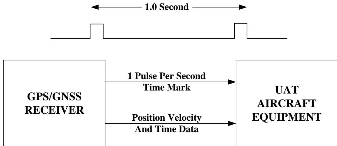
Figure 5-2: UAT Interface to GPS/GNSS Receiver
