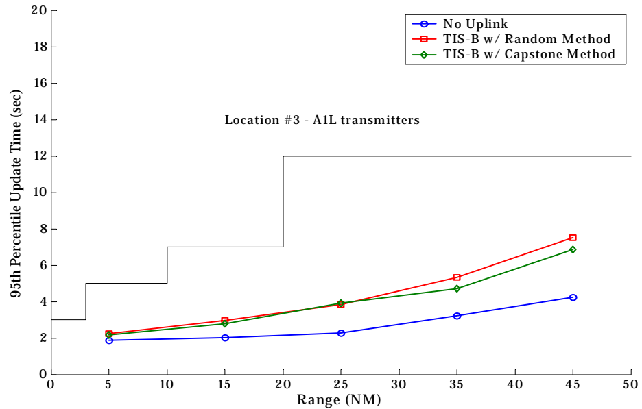
Figure B-40: ADS-B 95% Update Interval in Near-Term Scenario
