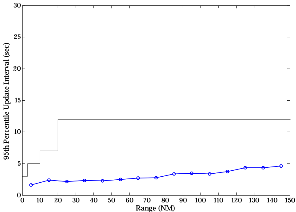
Figure B-34: A3 Receiver in Low Density Scenario Receiving A3 Transmissions
