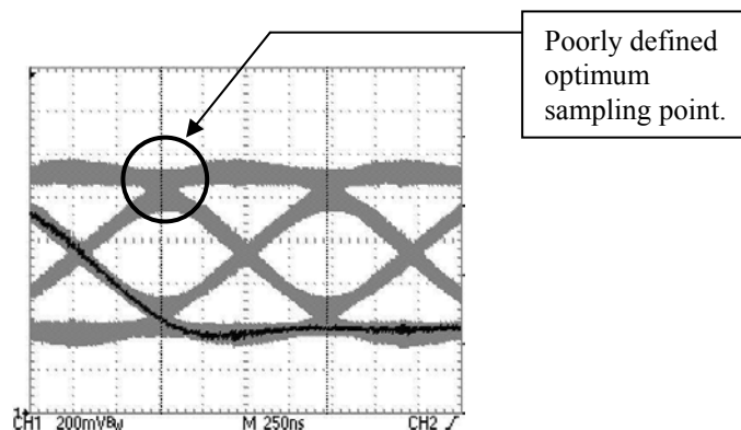
Figure A-2: Distorted eye diagram
