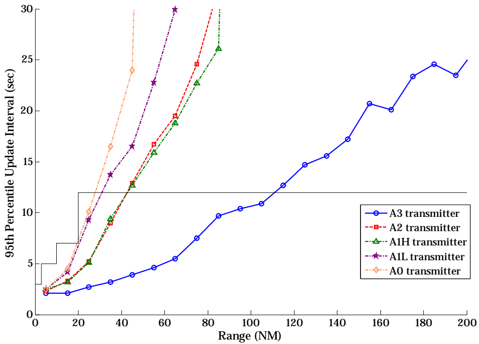
Figure B-28: Air-to-Air Reception by A1 Receiver at FL 150 over BRU in CE 2015
