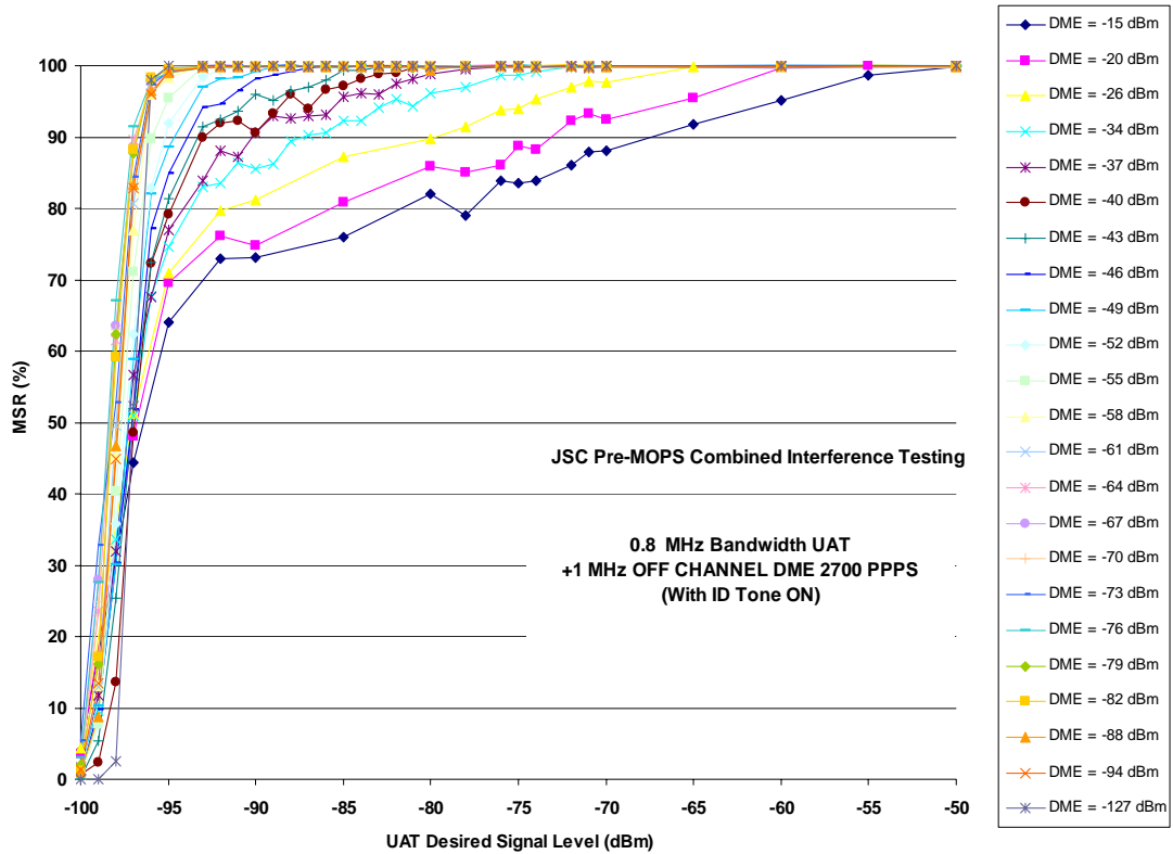
Figure D-5: UAT High Performance Receiver with DME 2700 Pulse Pairs at +1 MHz
