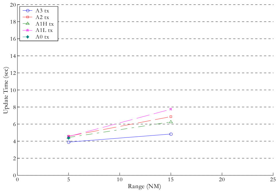
Figure B-37: A0 Receivers on the Ground in CE2015 Receiving All Aircraft on Approach at an Altitude of 2000 ft to Brussels co-located with a 10 kW 979 MHz TACAN
