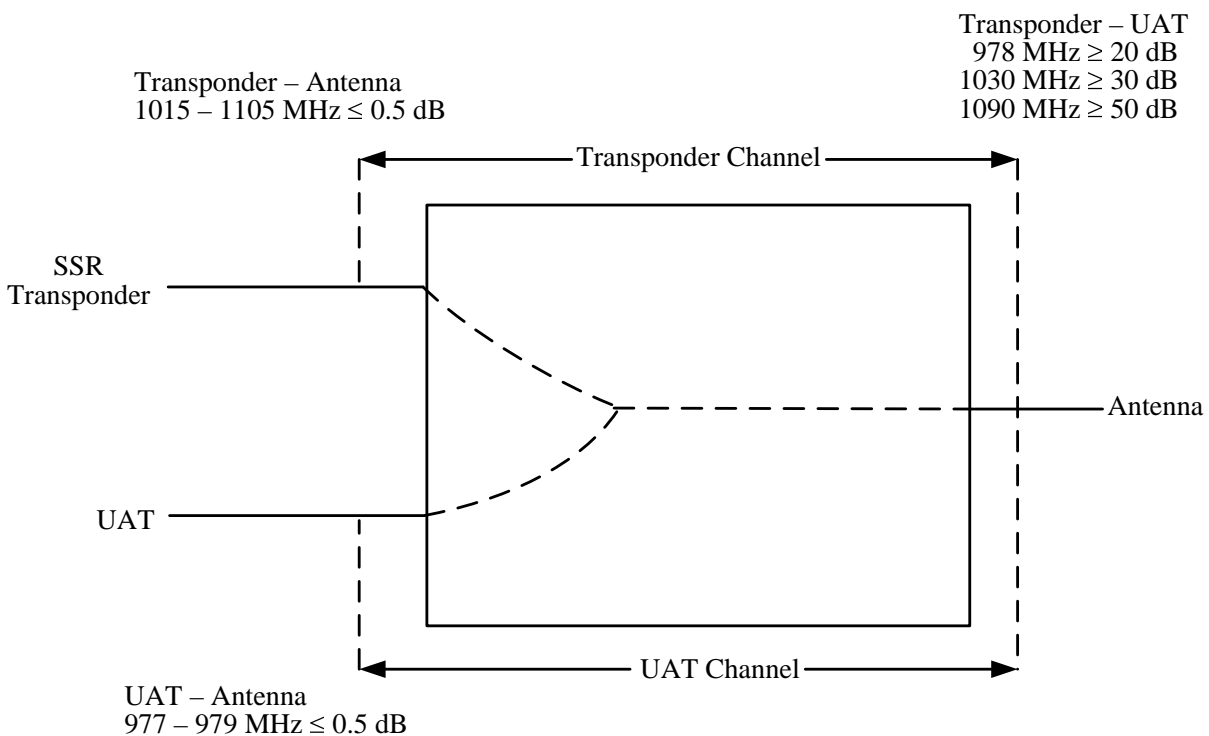
Figure 5-1: Optional Passive Diplexer Block Diagram
