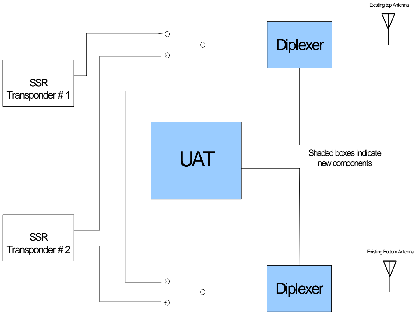
Figure H-10: Diplexer Installation
