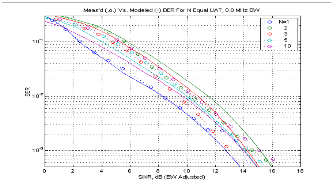
Figure B-10: N Equal UATs, INR \gg 0, 0.8 MHz Receiver
