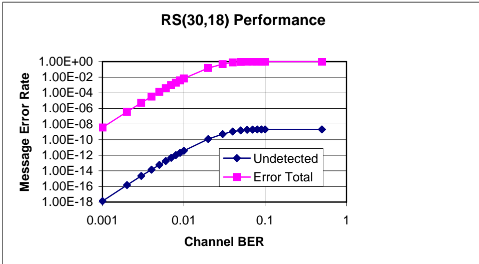
Figure E-1: Basic ADS-B Message Performance
