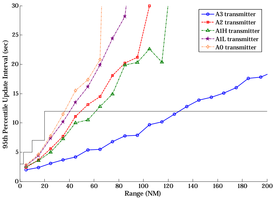
Figure B-14: Air-to-Air Reception by A3 Receiver at FL 150 over LA 2020
