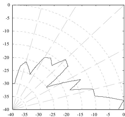
Figure C-2: Normalized DME Pattern
