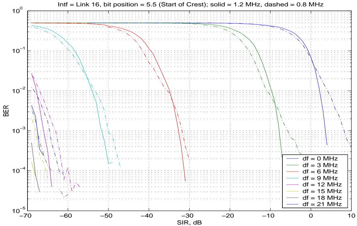
Figure B-6: Link 16 Interference
