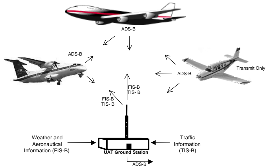
Figure 2-1: UAT Connectivity
