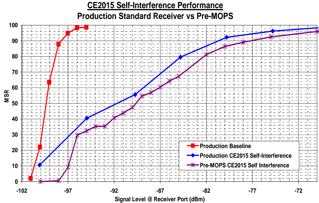
Figure D-17: UAT Production Standard Receiver Performance Comparison with the Core Europe 2015 Self-Interference Scenario
