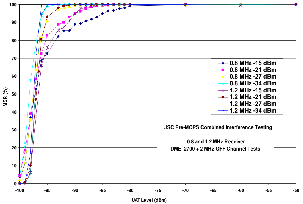
Figure D-3: UAT Receiver Performance DME 2700 Pulse Pairs at +2 MHz
