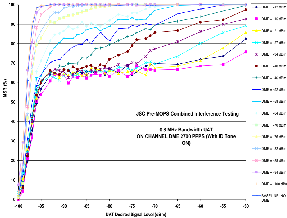
Figure D-7: UAT High Performance Receiver DME 2700 Pulse Pairs on Frequency
