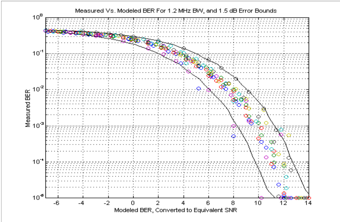
Figure B-11 Model Errors for All Data, 1.2 MHz Receiver
