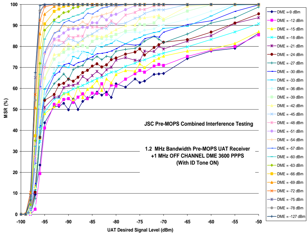
Figure D-10: UAT Standard Receiver Performance DME 3600 Pulse Pairs at +1 MHz
