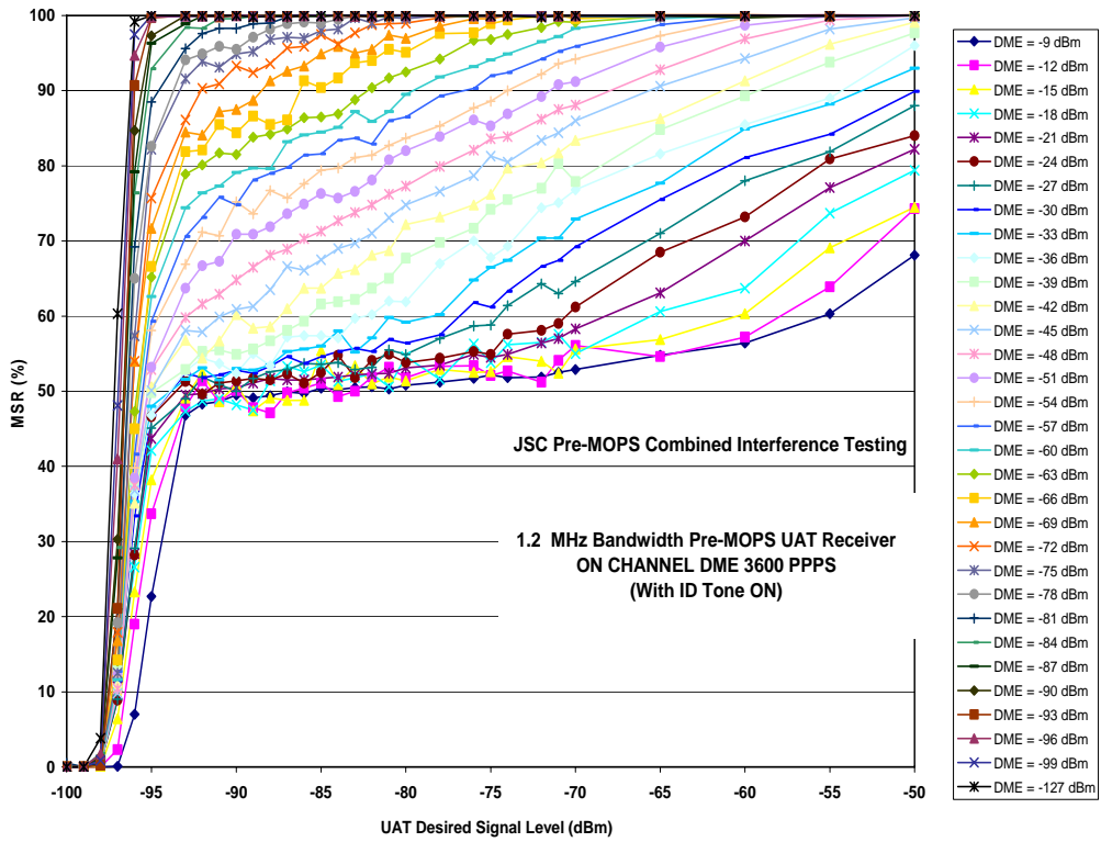
Figure D-12: UAT Standard Receiver Performance DME 3600 Pulse Pairs On Frequency
