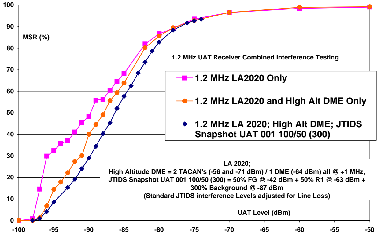
Figure B-47: Bench Test Measurements of UAT Performance in the LA2020 UAT Self-Interference, Combined with DME/TACAN and Link 16 Interference
