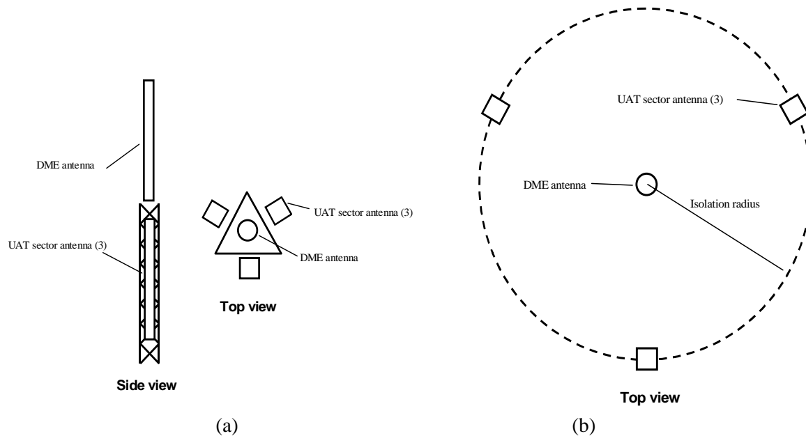
Figure 6-8: Possible UAT Ground Station Antenna Geometries
