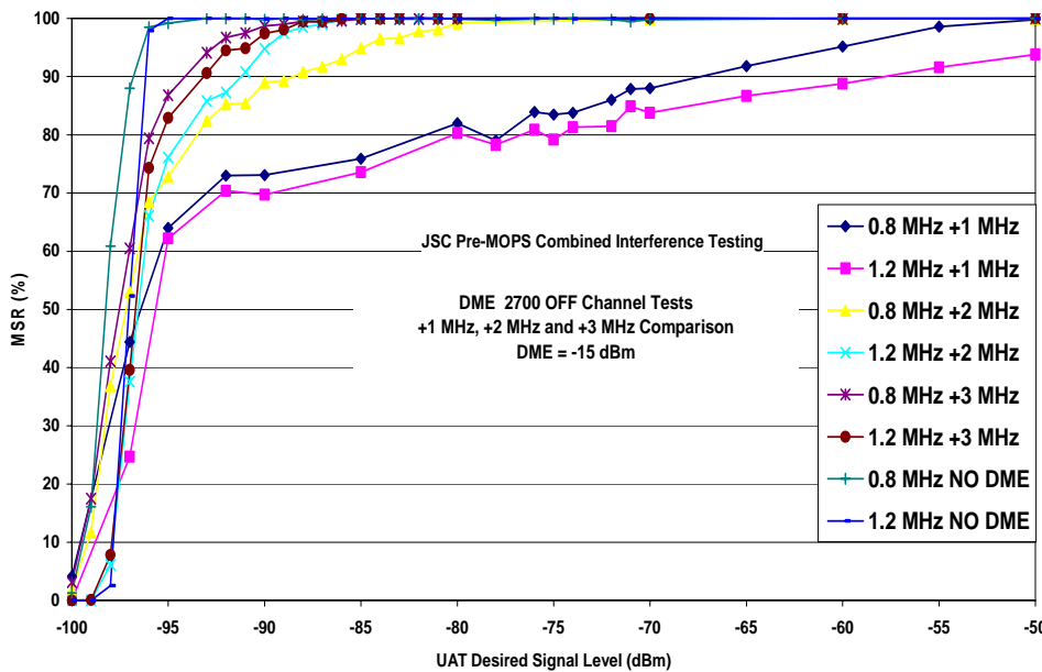
Figure D-14: UAT Receiver Performance DME 2700 Pulse Pairs Offset in Frequency
