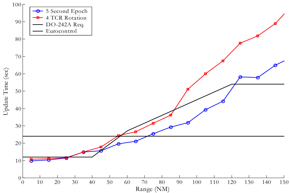
Figure I-3: 95th Percentile Target Change Report Update Times for an A3 Receiver at High Altitude in CE 2015 over Brussels Comparing Both Methods for Delivering 4 TC Messages
