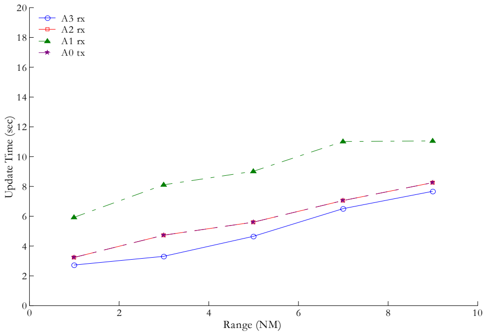
Figure B-33: Reception of Ground Vehicle Transmissions by Aircraft on Approach at 2000 feet into BRU in 2015 with 10 kW 979 MHz TACAN at Airport
