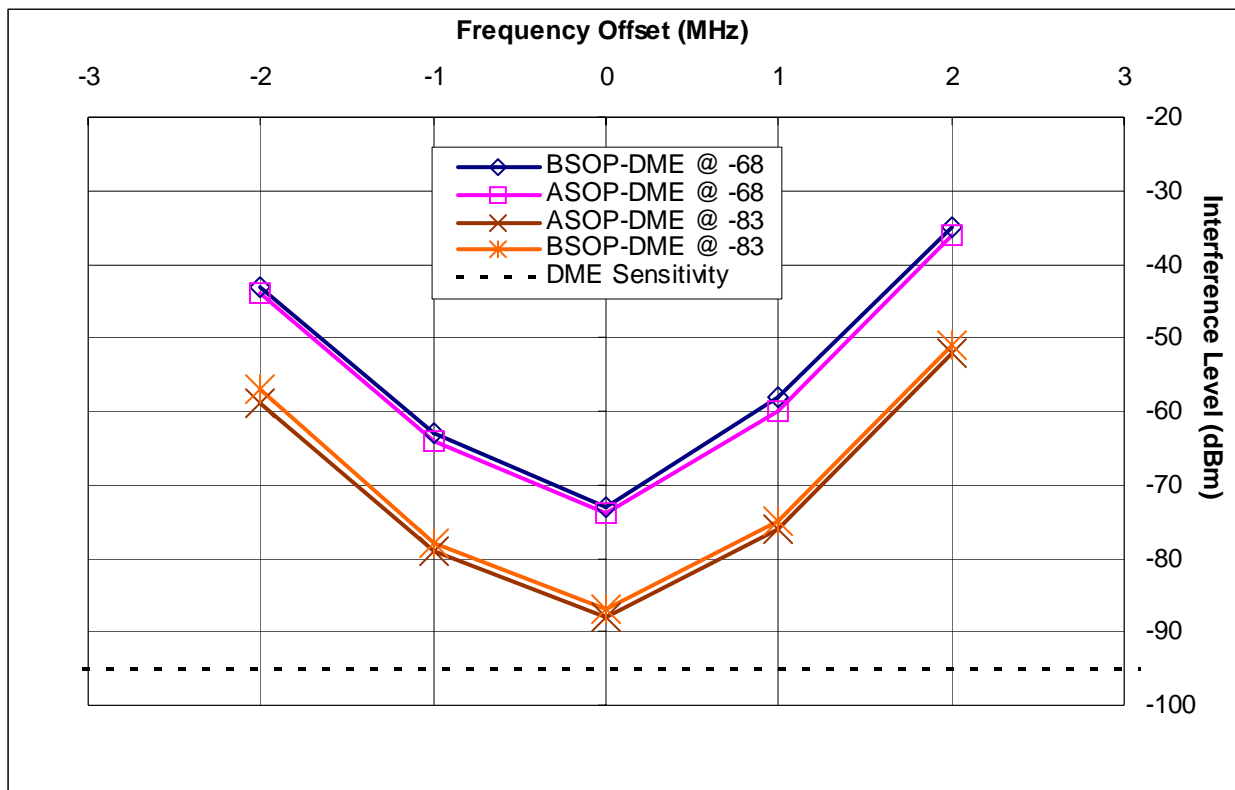
Figure F-1: Bendix King KD-7000 Frequency Offset Test
