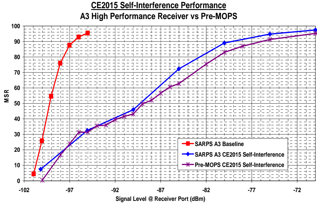
Figure D-18: UAT A3 Receiver Performance Comparison with the Core Europe 2015 Self-Interference Scenario
