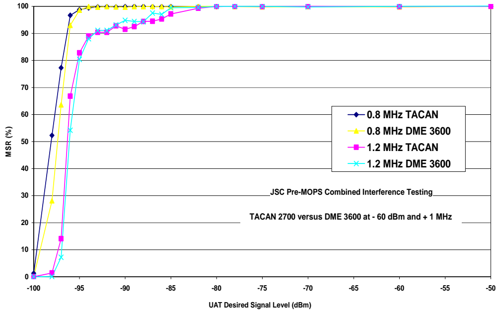
Figure D-15: UAT Receiver Performance TACAN 2700 and DME 3600 Pulse Pairs at +1 MHz
