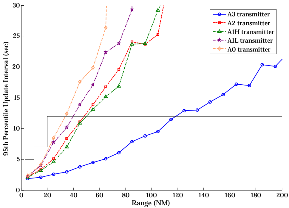
Figure B-24: Air-to-Air Reception by A3 Receiver at FL 150 over BRU in CE 2015
