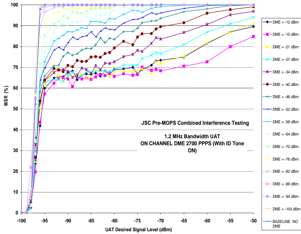
Figure D-6: UAT Standard Receiver Performance DME 2700 Pulse Pairs On Frequency
