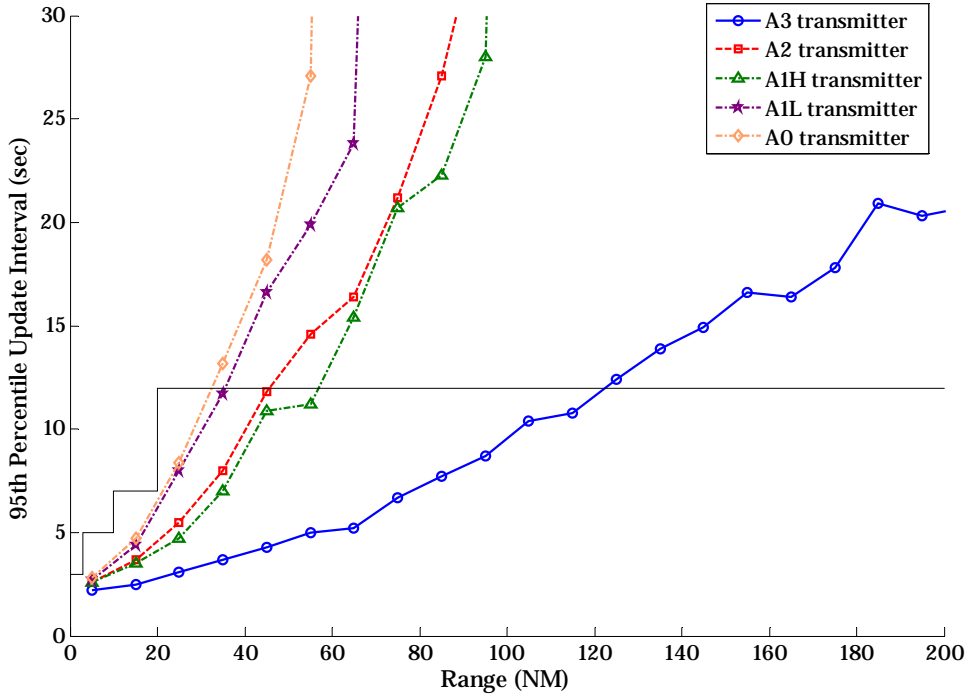
Figure B-18: Air-to-Air Reception by A1 Receiver at FL 150 over LA 2020
