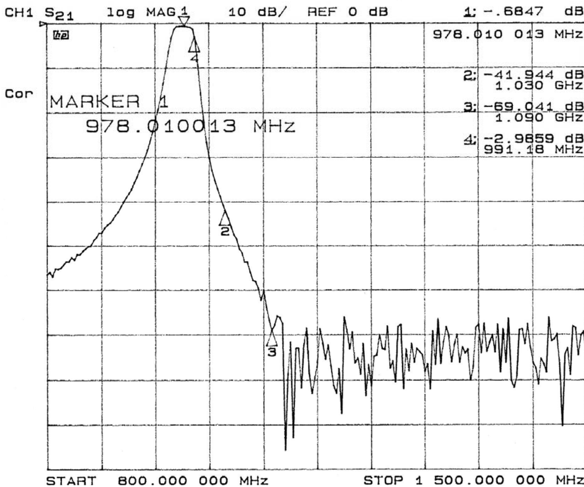
Figure H-7: Diplexer UAT Port
