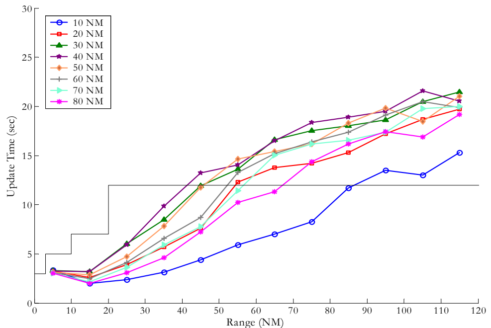
Figure B-42: 95% State Vector Update Times for an A3 Receiver at 40,000 feet Receiving A3 Transmissions in the Presence of a Ground Station at Various Ranges Broadcasting 1000 TIS-B Messages Per Second
