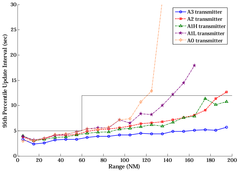
Figure B-20: Air-to-Ground Reception by a Receiver at LAX in LA 2020
