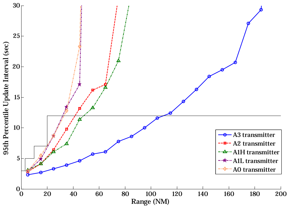
Figure B-19: Air-to-Air Reception by A0 Receiver at FL 150 over LA 2020
