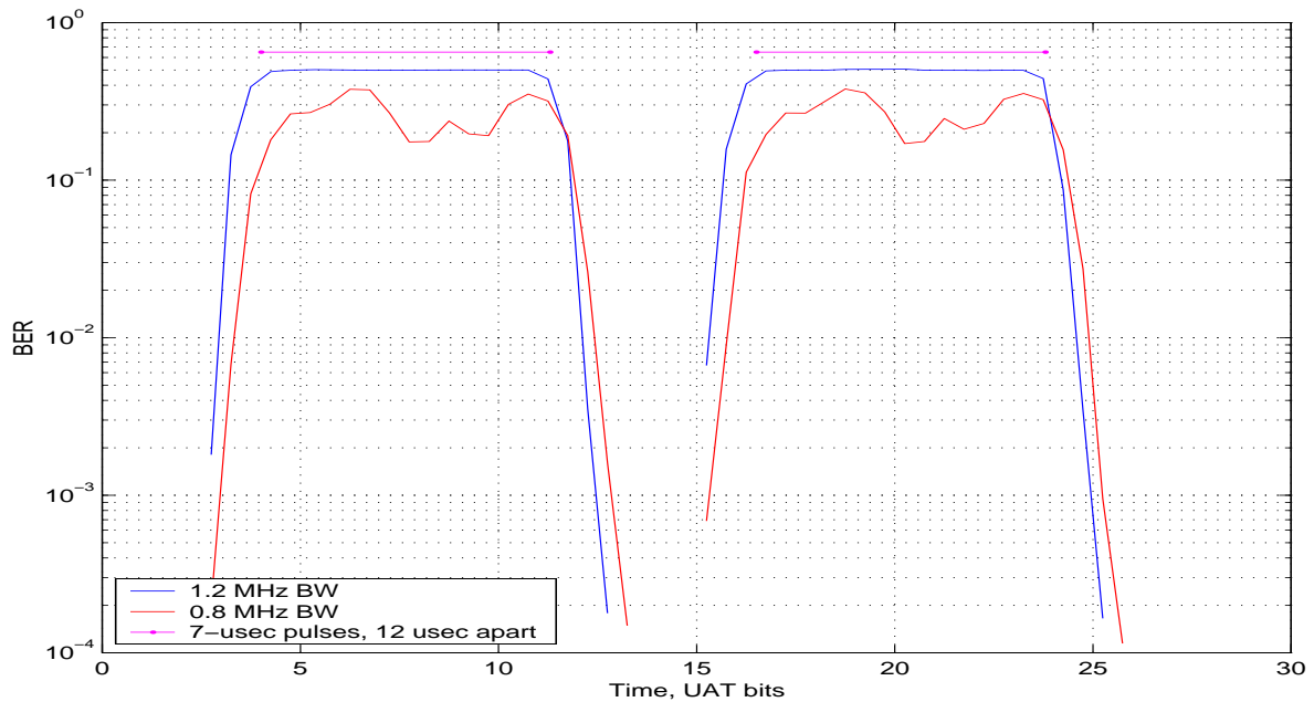
Figure B-5: BER Due to DME Interference
