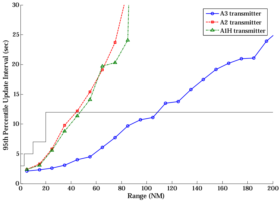
Figure B-27: Air-to-Air Reception by A1 Receiver at High Altitude over BRU in CE 2015
