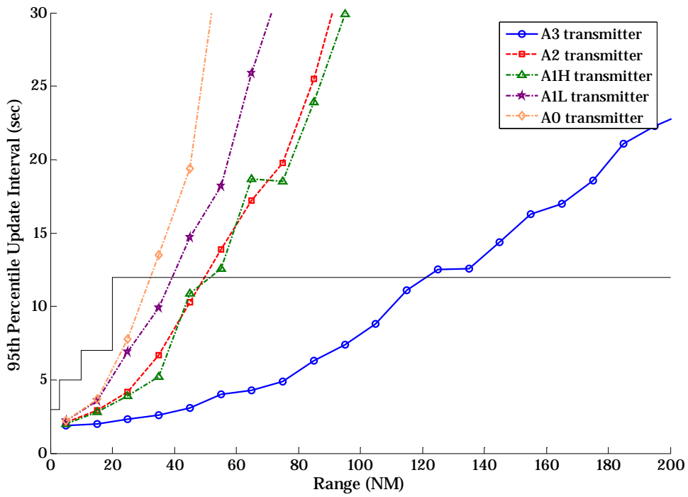
Figure B-26: Air-to-Air Reception by A2 Receiver at FL 150 over BRU in CE 2015
