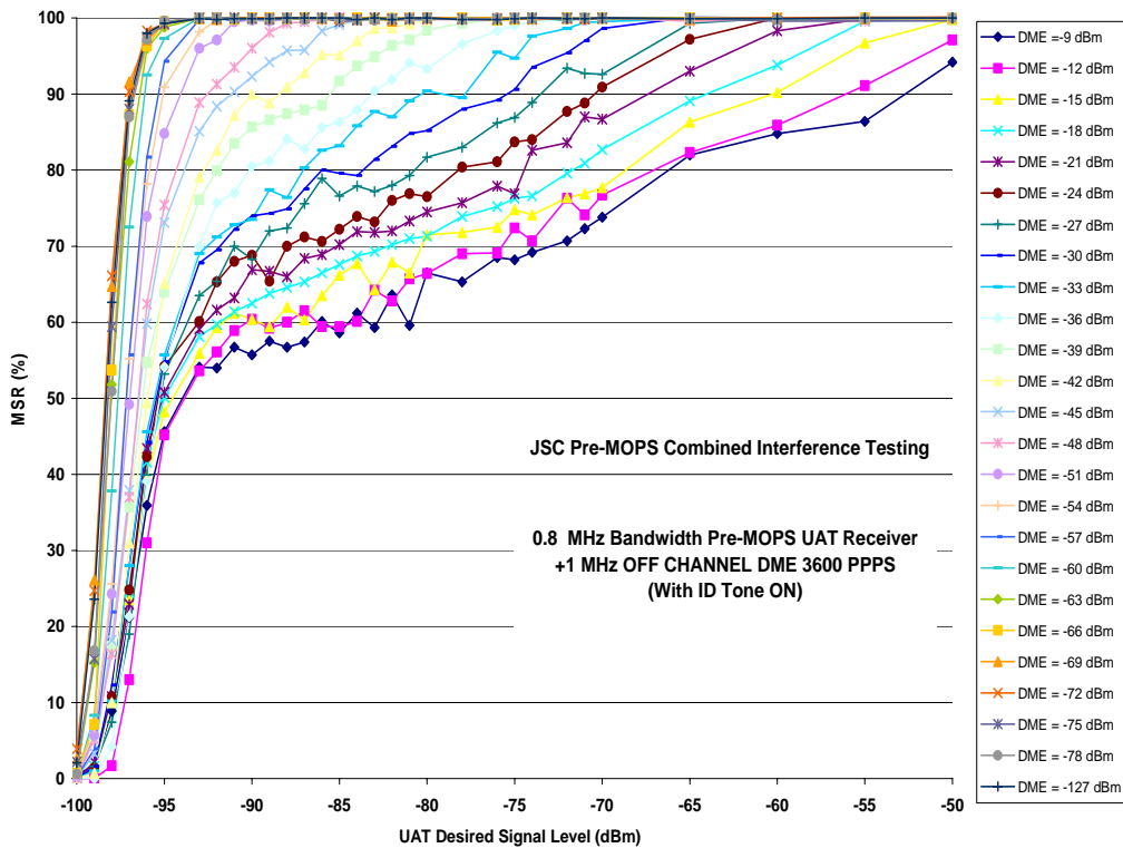
Figure D-11: UAT High Performance Receiver DME 3600 Pulse Pairs at +1 MHz
