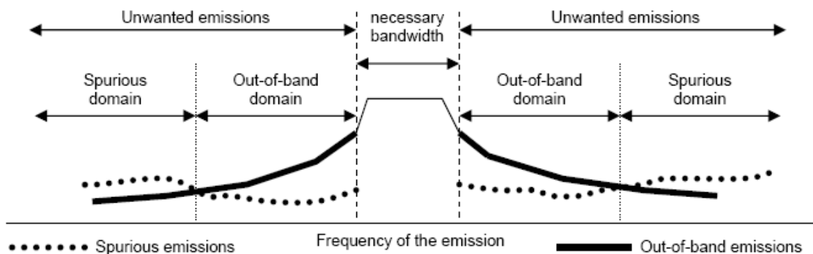
Figure 8-1: Unwanted Emissions and necessary Bandwidth
