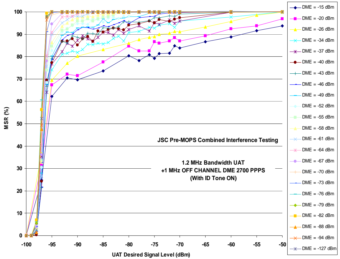
Figure D-4: UAT Standard Receiver Performance DME 2700 Pulse Pairs at +1 MHz
