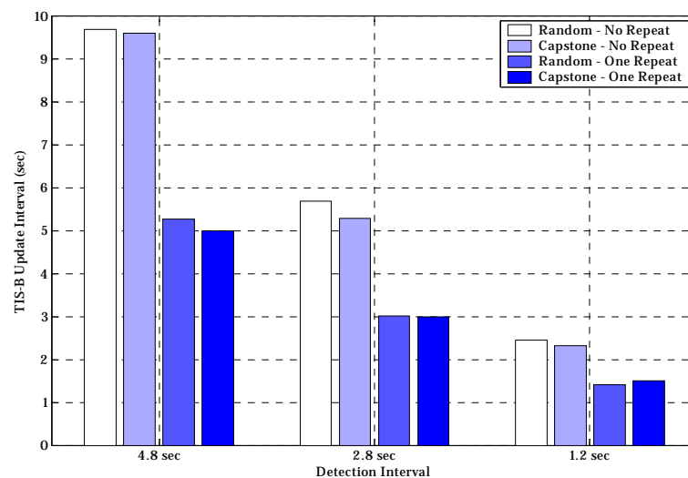
Figure B-39: TIS-B 95% Update Intervals in LA 2008 (No ADS-B Equipage)
