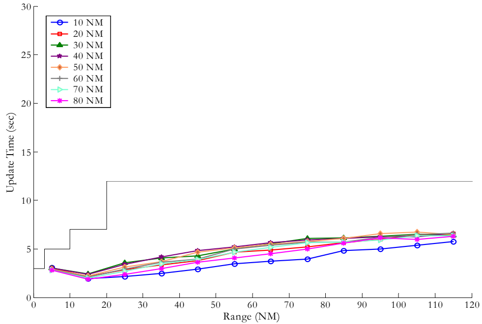
Figure B-43: 95% State Vector Update Times for an A3 Receiver at 40,000 feet Receiving A3 Transmissions in the Presence of a Ground Station at Various Ranges Broadcasting 500 RIS-B Messages Per Second
