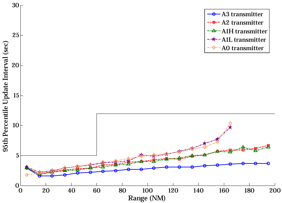
Figure B-31: Air-to-Ground Reception Using a 3-Sector Antenna at BRU in CE 2015
