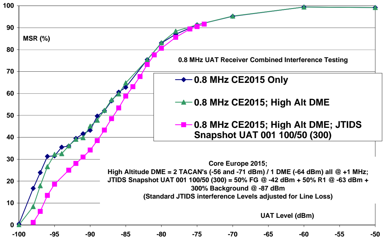
Figure B-46: Bench Test Measurements of UAT Performance in Core Europe UAT Self-Interference, Combined with DME/TACAN and Link 16 Interference
