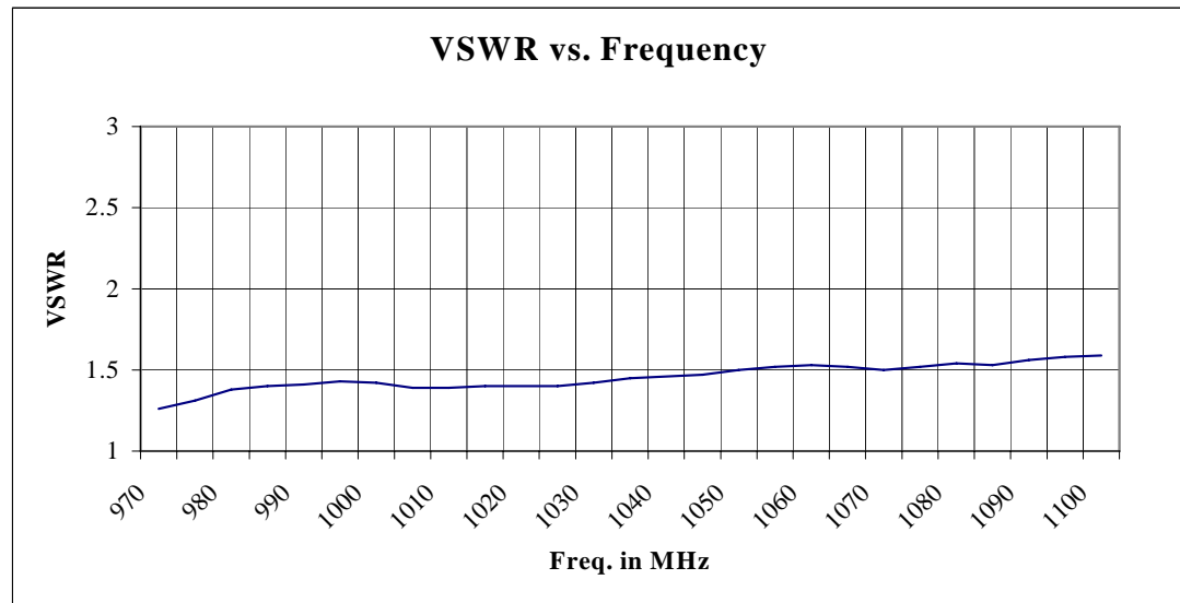
Figure H-5: ¼ Wave Whip Antenna
