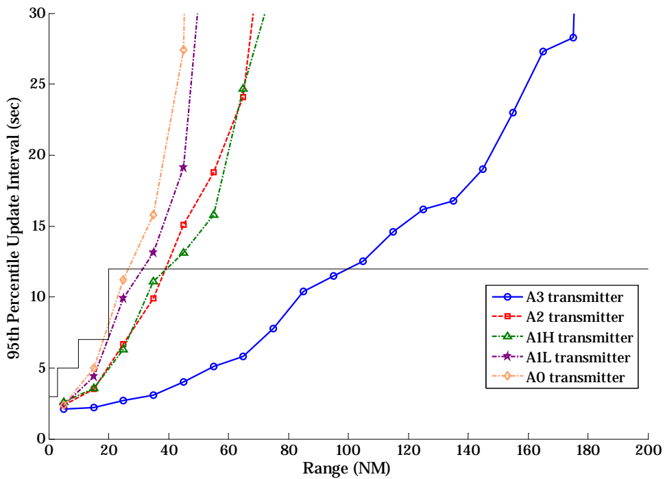
Figure B-29: Air-to-Air Reception by A0 Receiver at FL 150 over BRU in CE 2015
