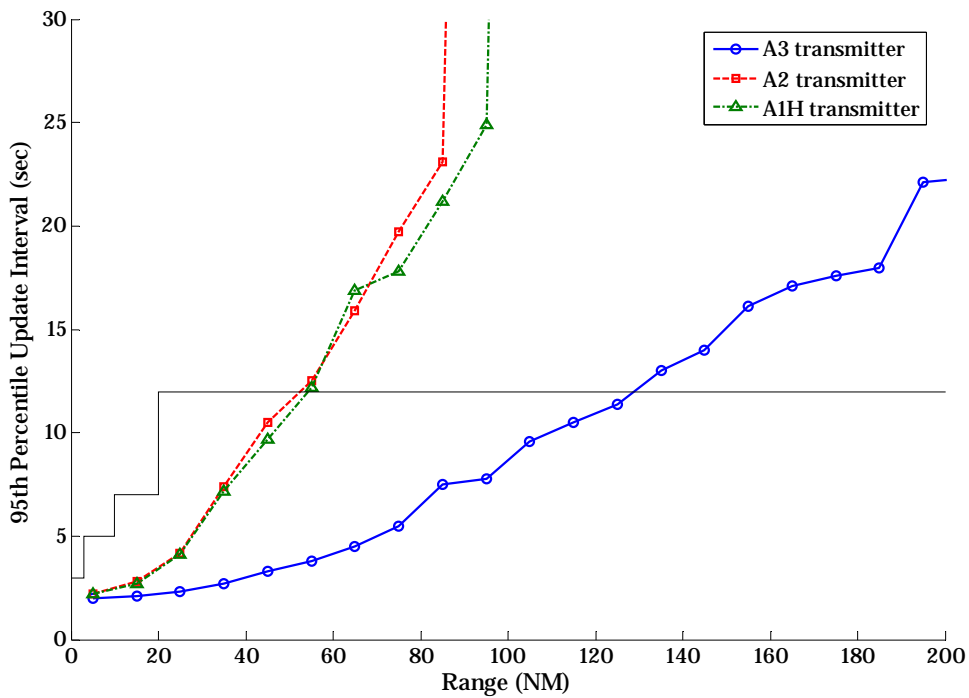
Figure B-25: Air-to-Air Reception by A2 Receiver at High Altitude over BRU in CE 2015
