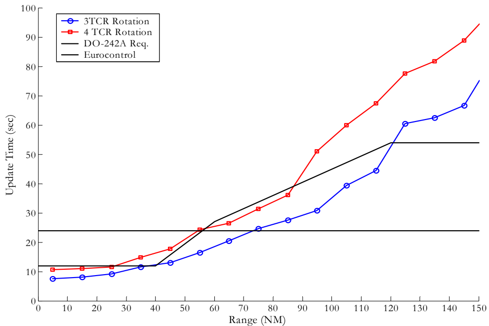
Figure I-1: 95th Percentile Trajectory Change Report Update Times for an A3 Receiver at High Altitude in CE 2015 over Brussels Using TC Rotation to Deliver Messages Containing Information for 3 or 4 TCRs
