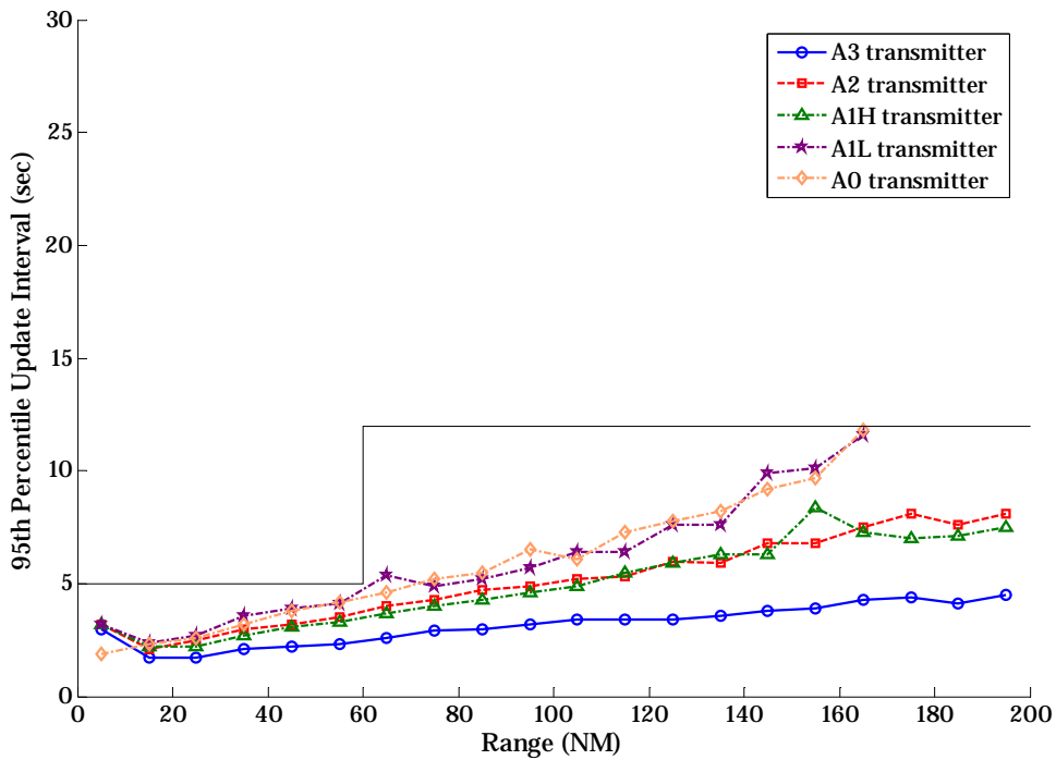
Figure B-32: Air-to-Ground Reception 2 NM from a 10 kW TACAN Using a 3-Sector Antenna at BRU in CE 2015
