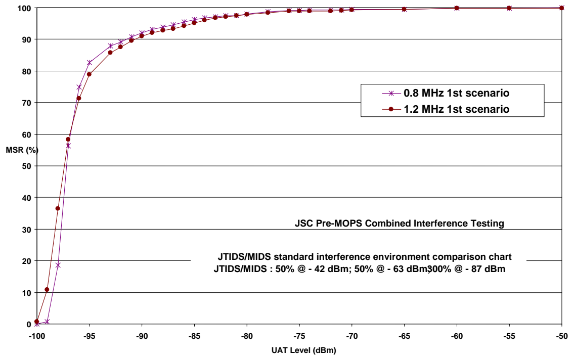
Figure D-16: UAT Receiver Performance with the first JTIDS/MIDS Scenario
