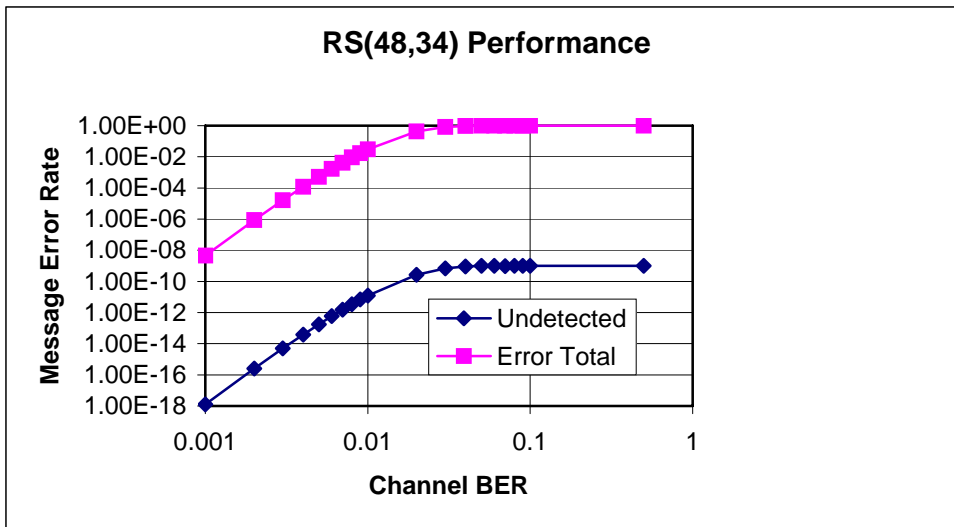
Figure E-2: Long ADS-B Message Performance
