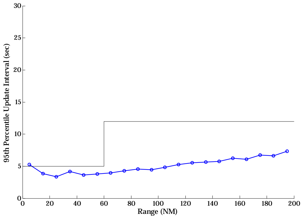
Figure B-35: Receptions of A3 Transmissions by a UAT Ground Receiver in a Low Density Scenario co-located with a TACAN at 979 MHz with -30 dBm Power at the UAT Antenna
