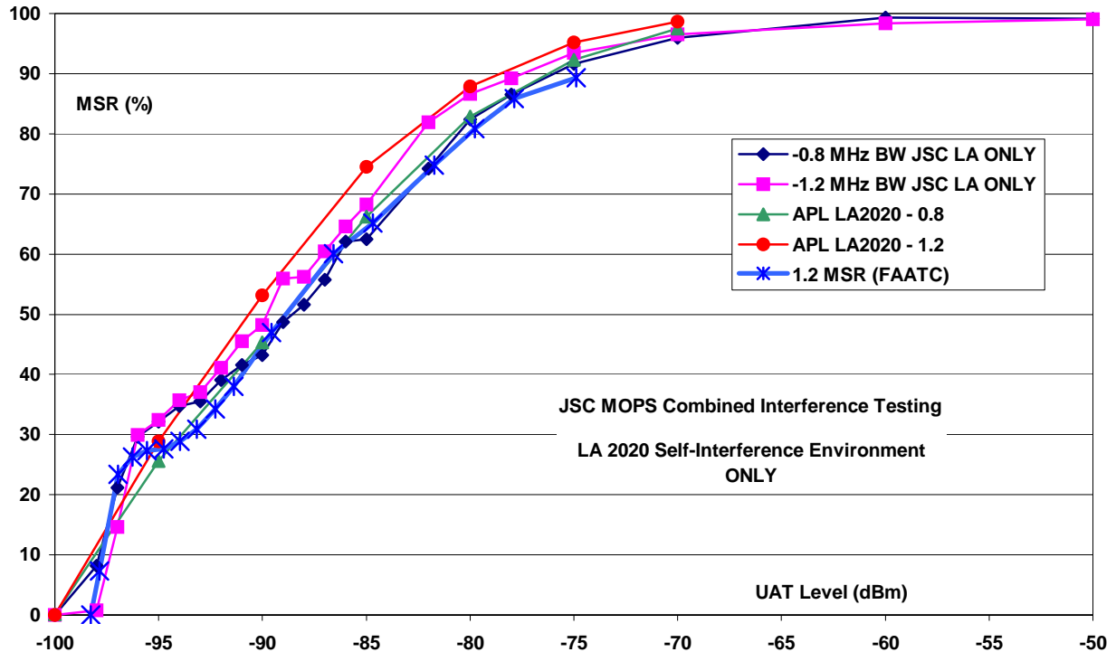
Figure B-45: Comparison of Bench Test Measurements of MOPS-Compliant UAT Reception in LA2020 Self-Interference with Predictions by MAUS
