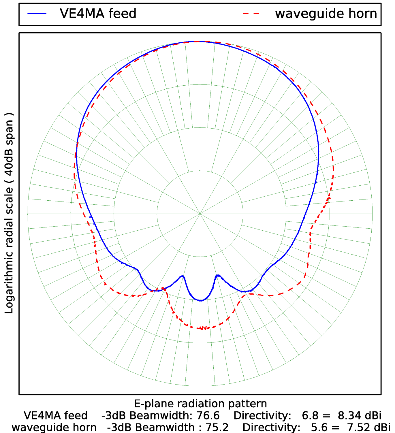
Figure 5: Measured feed E-plane radiation pattern.
