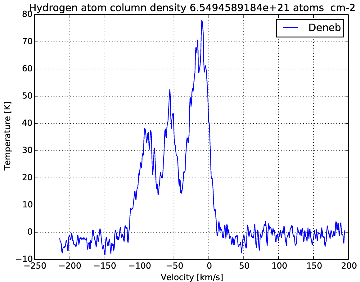
Figure 18: Neutral-hydrogen velocity and column density.
