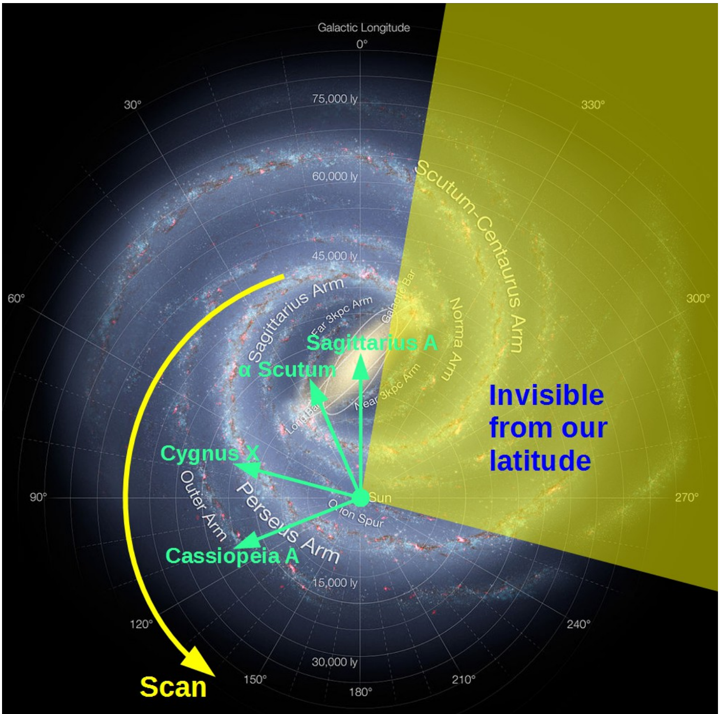
Figure 20: Galactic-plane scanning from our latitude.
