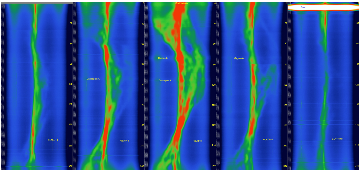
Figure 22: Measured 3D map of the Milky Way.
