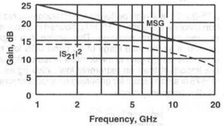
Insertion Power Gain and Maximum Stable Gain vs. Frequency V_{DS} = 1.5\text{ V}, I_{DS} = 20\text{ mA}
