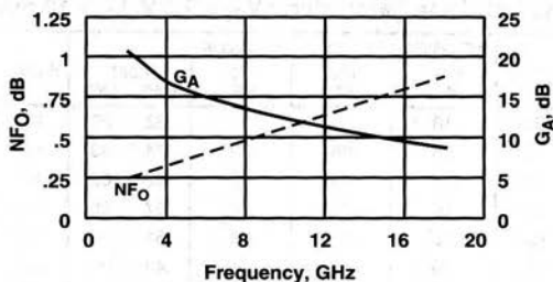
Noise Figure and Associated Gain vs. Frequency (ATF-35076) V_{DS} = 1.5\ \text{V} , I_{DS} = 10\ \text{mA}
