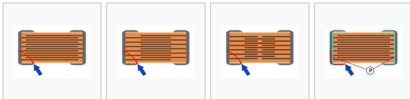
Standard MLCC chip, short circuit possible if ceramic breaks due to mechanical stress „Open-Mode-Design“ MLCC chip, a break only reduces the capacitance value "Floating-Electrode-Design"- MLCC, a break only reduces the capacitance value "Flex-Termination" - MLCC chips, a flexible contact layer prevents breaking of the ceramic. [27]
