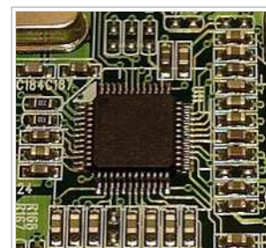
MLCCs as decoupling capacitors around a microprocessor
