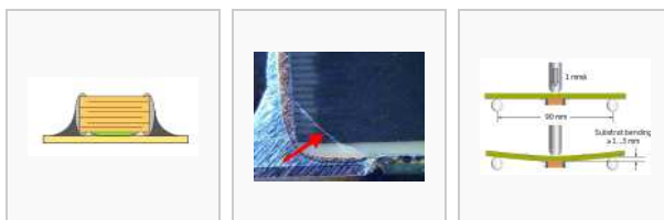
Correct mounted and soldered MLCC chip on a PCB Micrograph of broken ceramic in a MLCC chip Simplified figure of a bending test for soldered MLCC
