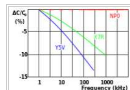
Frequency dependence of capacitance for ceramic X7R and Y5V class 2 capacitors (curve of NP0 class 1 for comparison)
