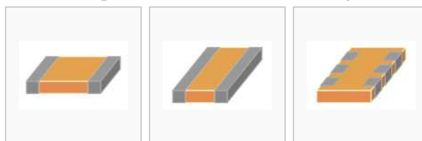
Standard MLCC chip design Low-ESL design of a MLCC chip MLCC chip array
