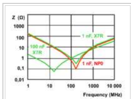
Typical curves of the impedance of X7R and NP0-MLCC-Chips
