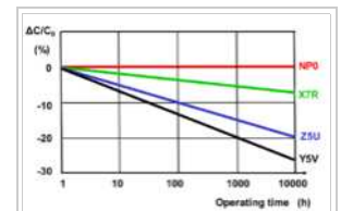
Aging of different Class 2 ceramic capacitors compared with NP0-Class 1 ceramic capacitor
