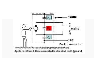
Appliance Class I capacitor connection
