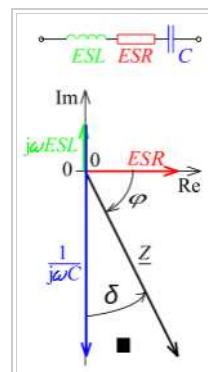
Simplified series-equivalent circuit of a capacitor for higher frequencies (above); vector diagram with electrical reactances X_{ESL} and X_C and resistance ESR and for illustration the impedance Z and dissipation factor \tan \delta
