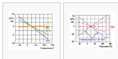
Idealized curves of different class 1 ceramic capacitors representation of the tolerance range of temperature coefficient \alpha
