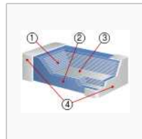
Detailed construction of a multilayer ceramic chip capacitor (MLCC). 1. Ceramic dielectric, 2. Ceramic or lacquered coating, 3. Metallized electrode, 4. Connecting terminals
