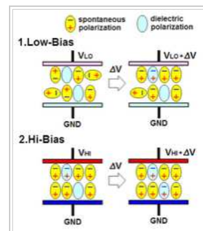
DC Bias characteristic of ferroelectric ceramic materials
