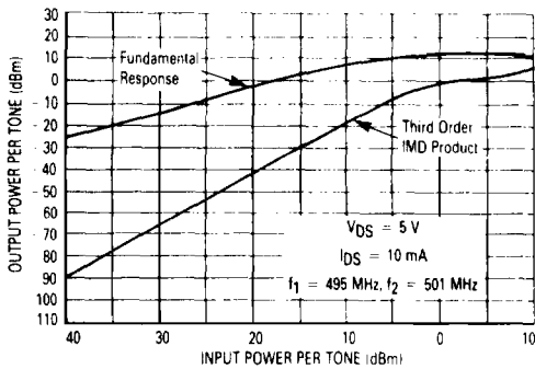
Figure 9. Third Order Intermodulation Distortion (α 500 MHz)
