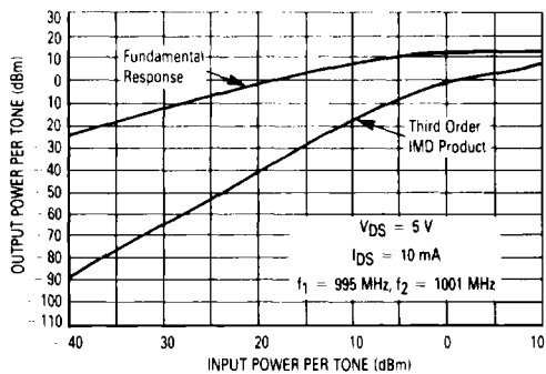
Figure 10. Third Order Intermodulation Distortion (α 1 GHz)
