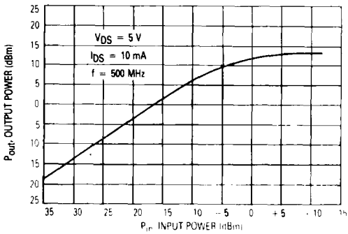
Figure 7. Output Power versus Input Power (α 500 MHz)
